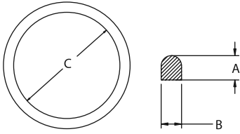
"D"-RINGS
